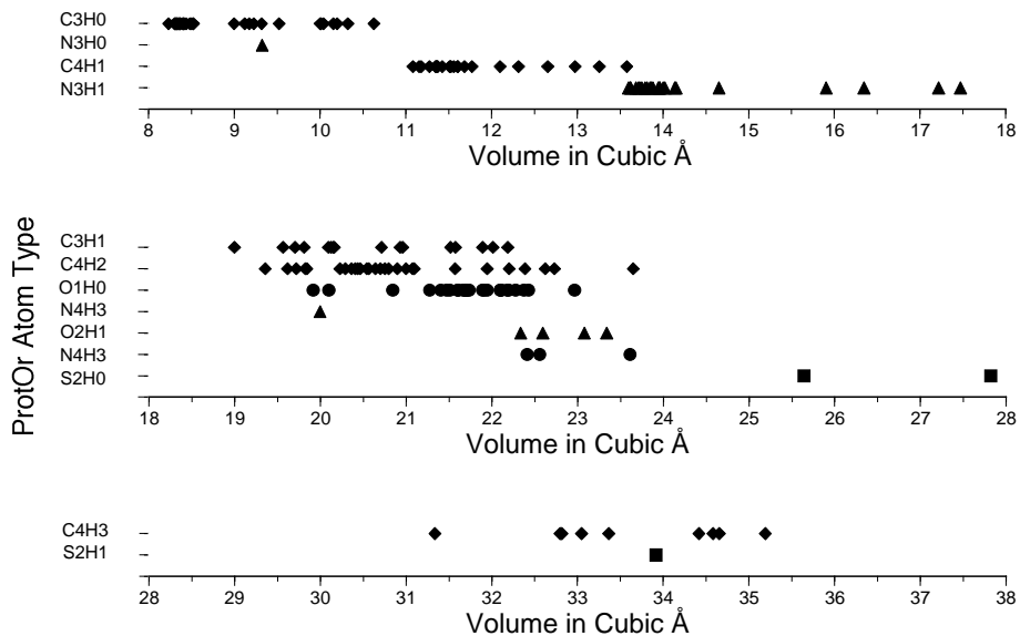
Fig. 4. Distribution of the raw 173 reference volumes. The 173 raw, reference volumes are shown based on their volume. For clarity, the graph is broken up into three 10 Å 3 segments along the x -axis. Also, atoms belonging to different chemical atom types are separated along the y -axis and a consistent symbol for each heavy atom type is used—diamonds for carbons, triangles for nitrogens, circles for oxygens, and squares for sulfurs.
