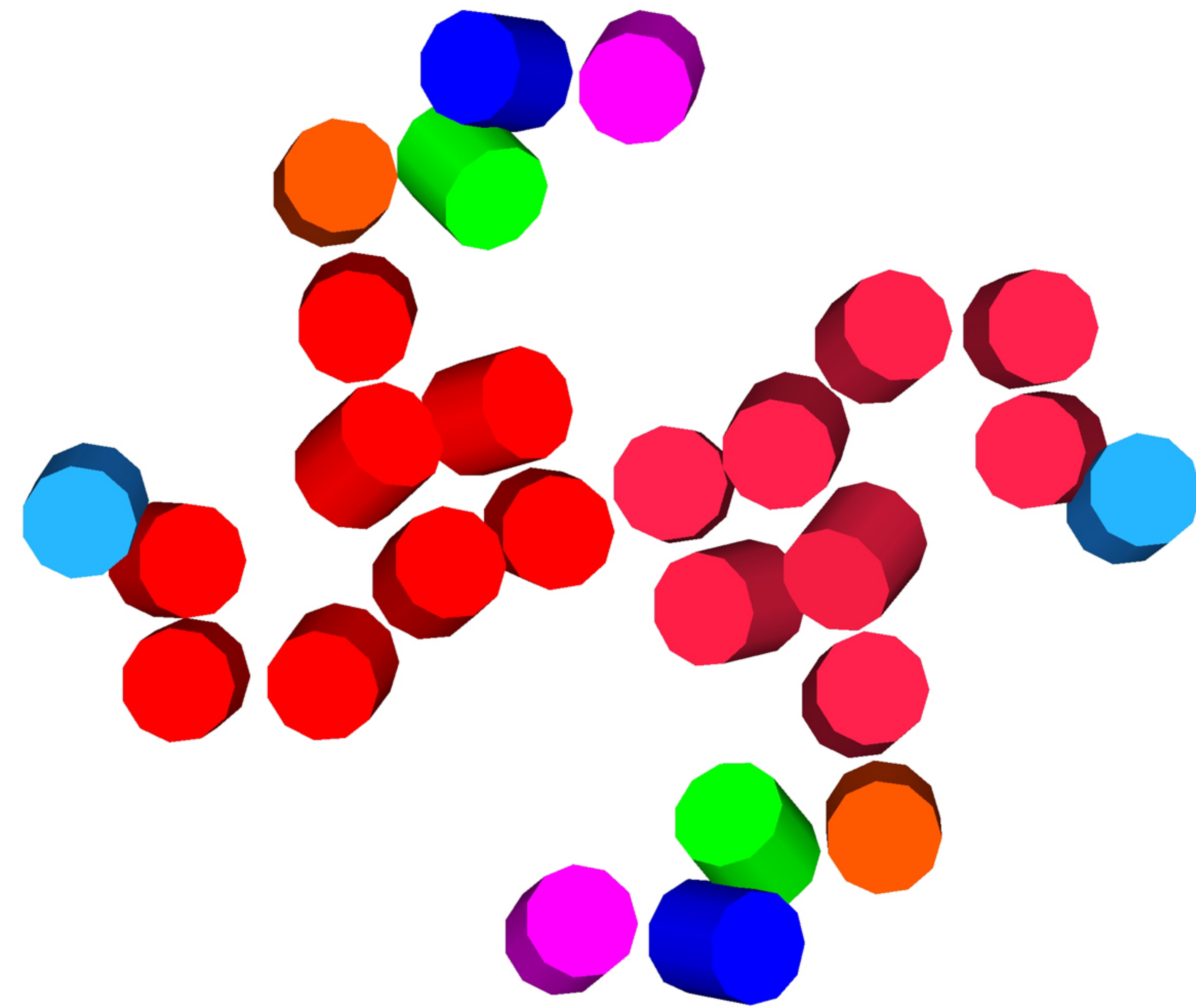
Cytochrome bc1 Complexes in bovine heart mitochondria Iwata et al. (1998)
