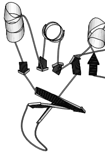
FAD Binding
