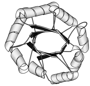
TIM Barrel
