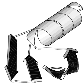
Beta-Grasp Fold
