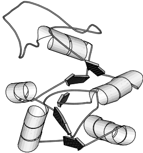
P-loop Hydrolase
