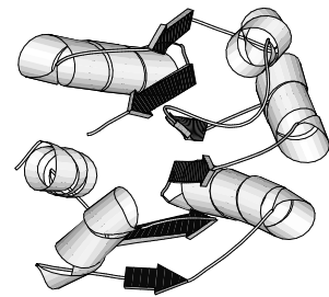
Thiamin Binding
