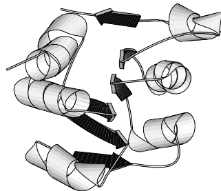
Rossmann Fold
