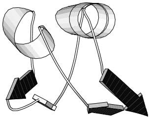
Ferredoxin Fold
