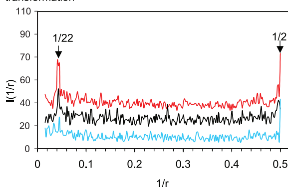
B. Periodicities in the distributions determined by Fourier transformation
