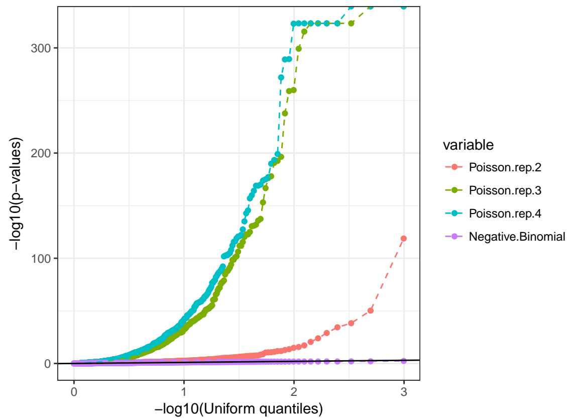
Quantile-quantile plot for mouse 18S rRNA DMS stop counts
