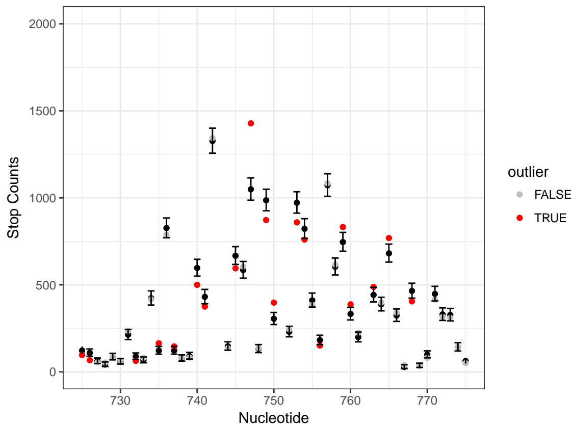
Observed replicates of mouse 18S rRNA DMS stop counts
