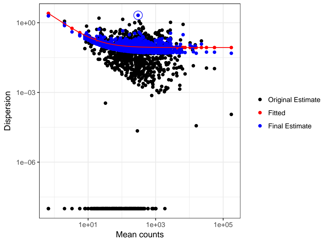
Dispersion estimates for mouse 18S DMS stop counts
