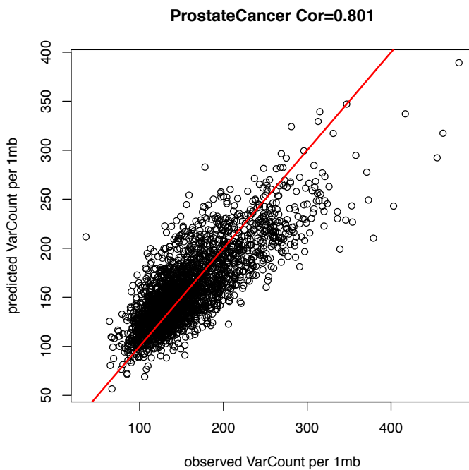
Figure S 2-11, (TL, #) BMR estimation with unmatched data
