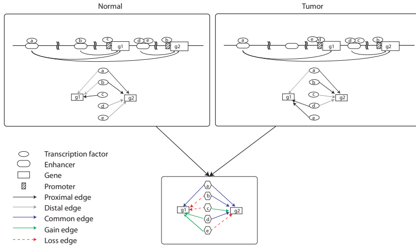
Figure S 5-1. (HL, II) Network rewiring schematics
