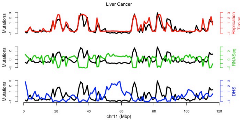
Figure S 2-3 (TL, ll) Example of external effects on local mutation rate
