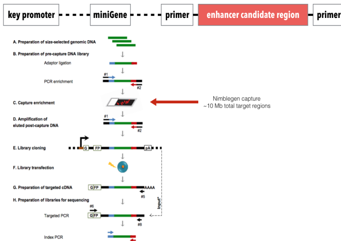
Figure S 3-7 (TL, †) Capture STARR-seq experiment design
