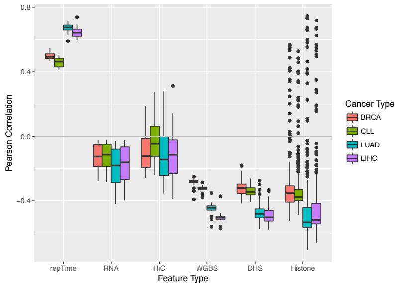
Figure S 2-4 (TL, ||) Correlation of mutation rate and external features across multiple cancer types (shadow figure for Fig. 2B)
