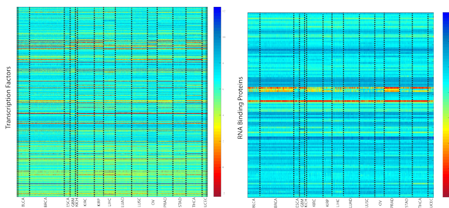
Figure S 4-1 (TL, ¶) Expression patterns of transcription factors across cancer types
