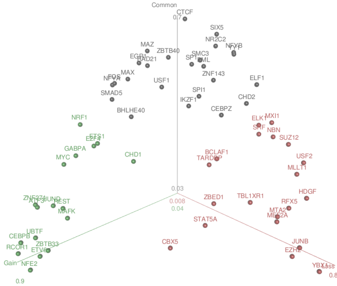
Figure S 5-2, (TL, II) Kmeans clustering of rewired TFs in K562 and GM12878
