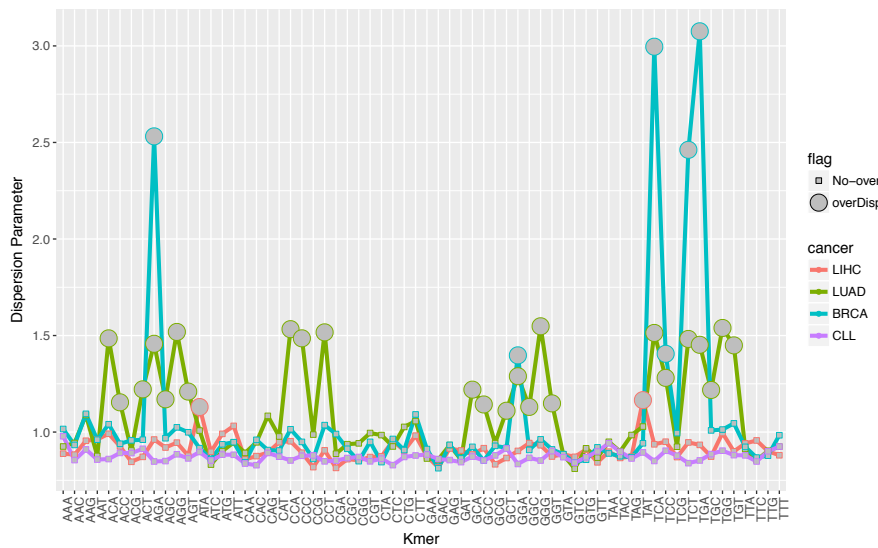
Figure S 2-9 (TL, #) Summary of estimated overdispersion parameter in multiple cancer types
