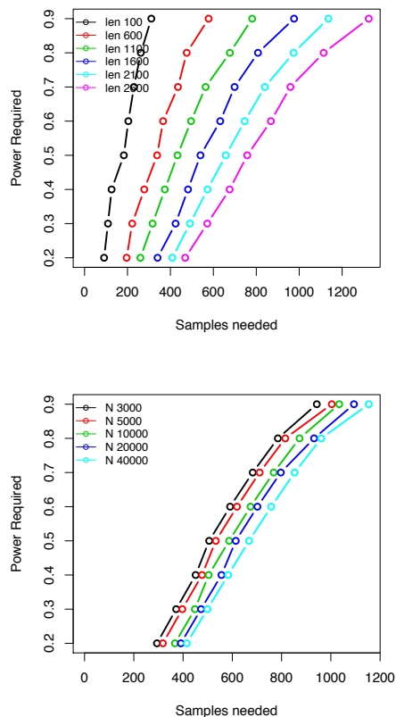
Figure S 3-1 (TL, II) Power analysis of annotation length effect
