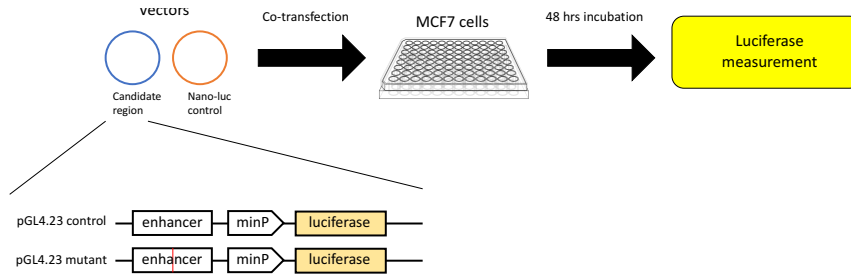
Figure S 6-3 (TL, ||) Schematic of SNV validation
