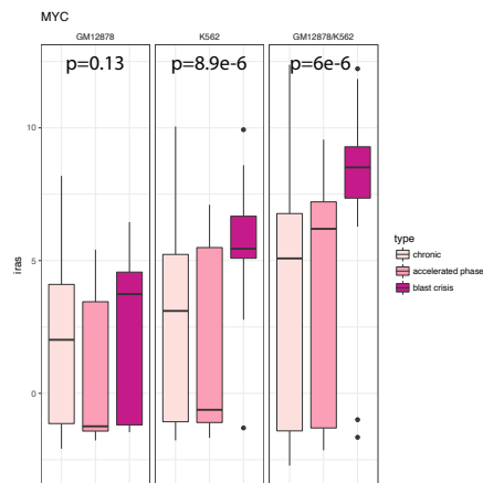
Figure S 5-11 (TL, II) MYC activity scores were then compared between three different severity levels using ANOVA
