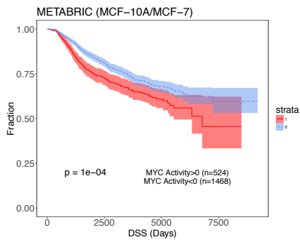
Figure S 5-8 (TL, II) Survival analysis on MYC's MCF-7 specific target genes
