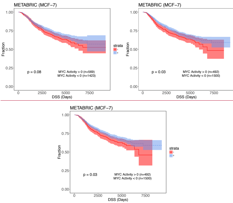
Figure S 5-10 (TL, ||) Survival analysis on MYC's target gene expression levels in three replicates
