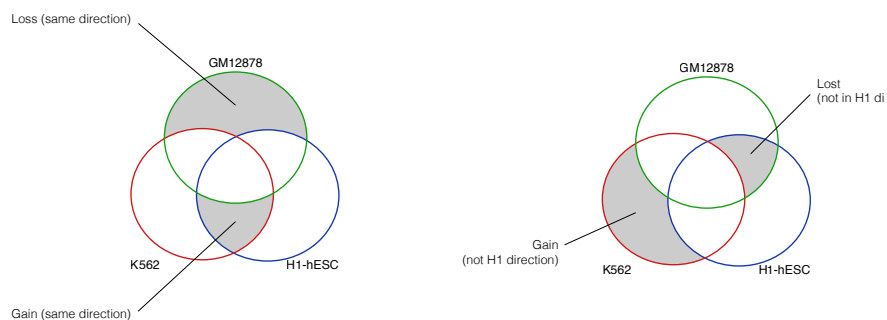
Figure S 5-5 (TL, ||) Comparison of rewiring direction with respect to H1-hESC
