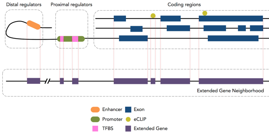
Figure S 3-12 (HL, ||, shadow figure for Fig. 2 C) Schematic of extended gene definition
