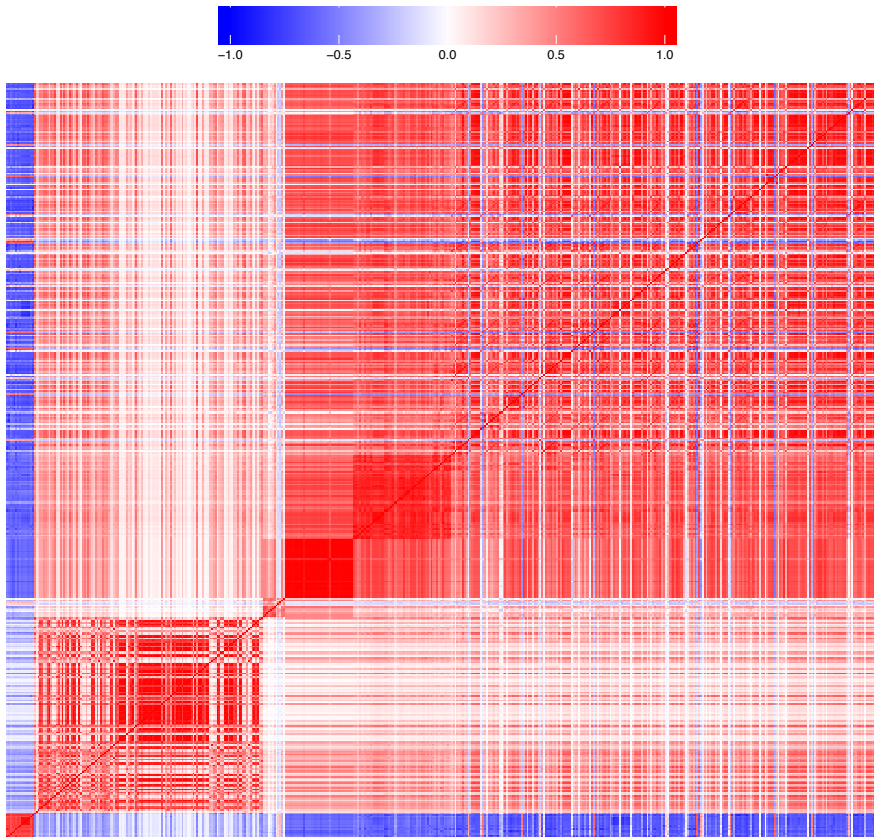
Figure S 2-6 (TL, #) Heatmap of feature correlations
