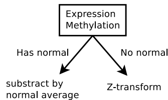
Figure S 1-8 (TL, II) Schematics of RNA-seq data processing
