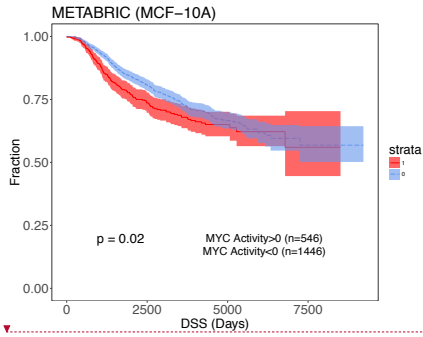
Figure S 5-10 (TL, ||) Survival analysis on MYC's target gene expression levels in three replicates
