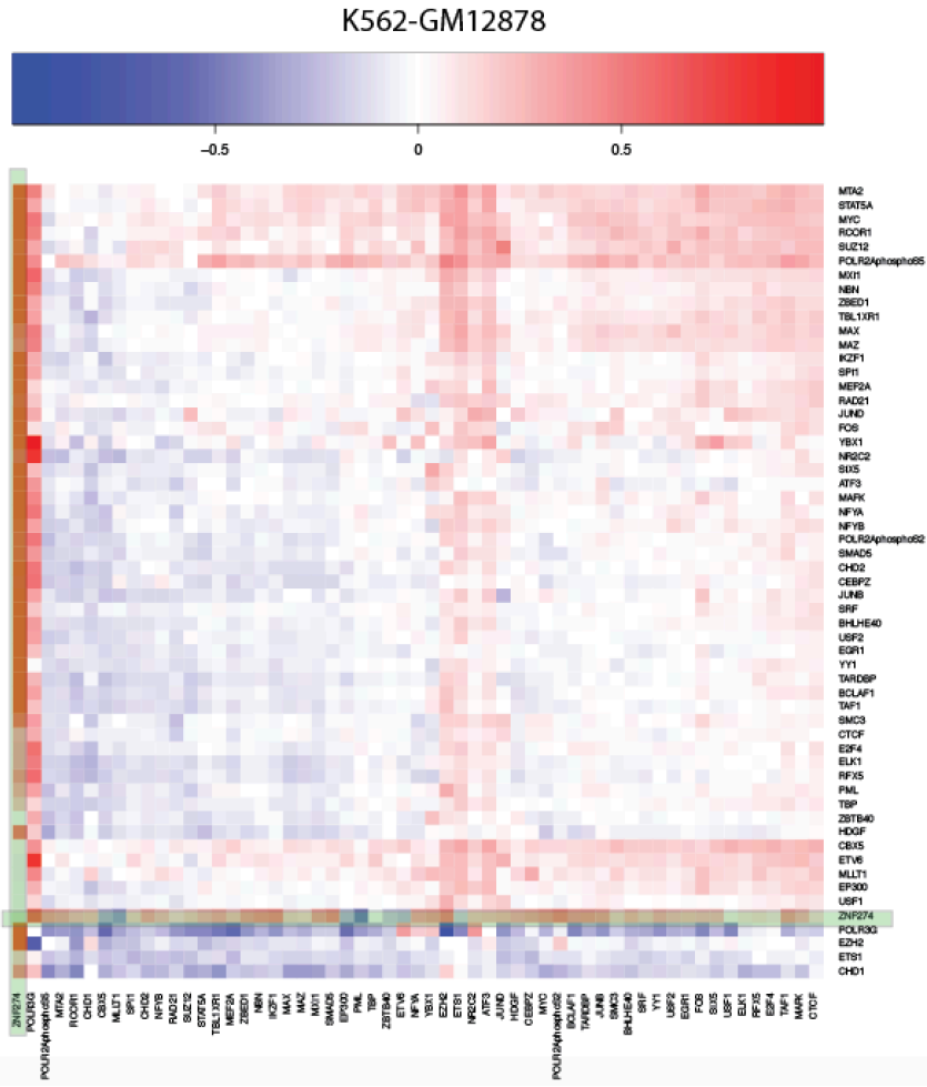
Figure S 5-14 (TL) Difference of co-binding scores c(i,j) of the transcription factors between K562 and GM12878 cell lines. Rows represent TF i and columns represent TF j . ZNF274, which has consistently higher co-binding scores with other TFs in K562 cell line compared to GM12878 is highlighted.
