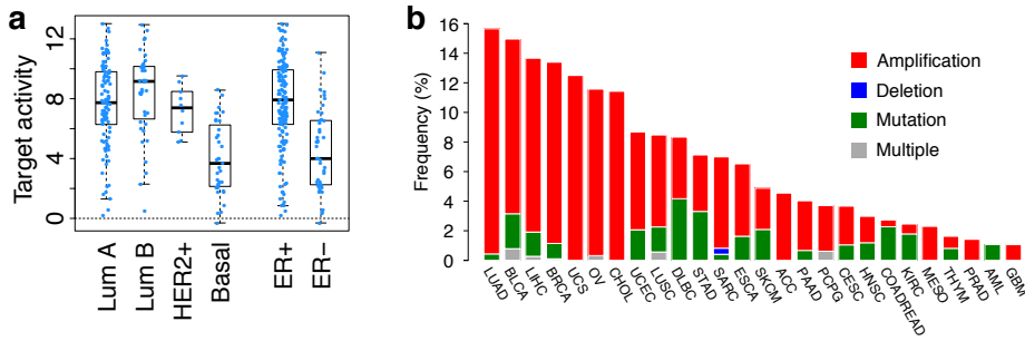
Figure S 4-5 (TL 2 ||) The potential role of ZNF687 in cancer
