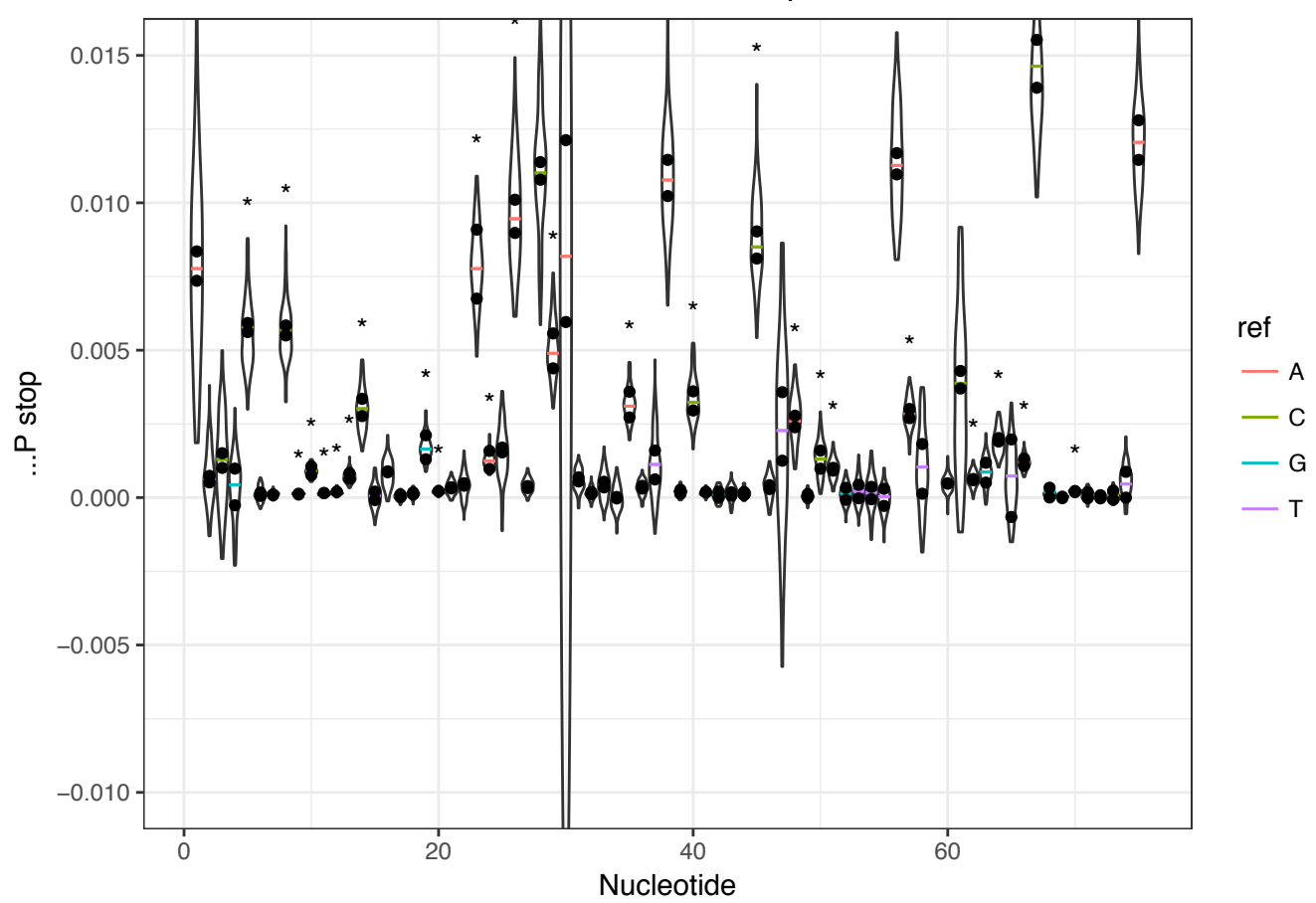
Inferred ...P distributions for mouse 7SK primer 1 stops
