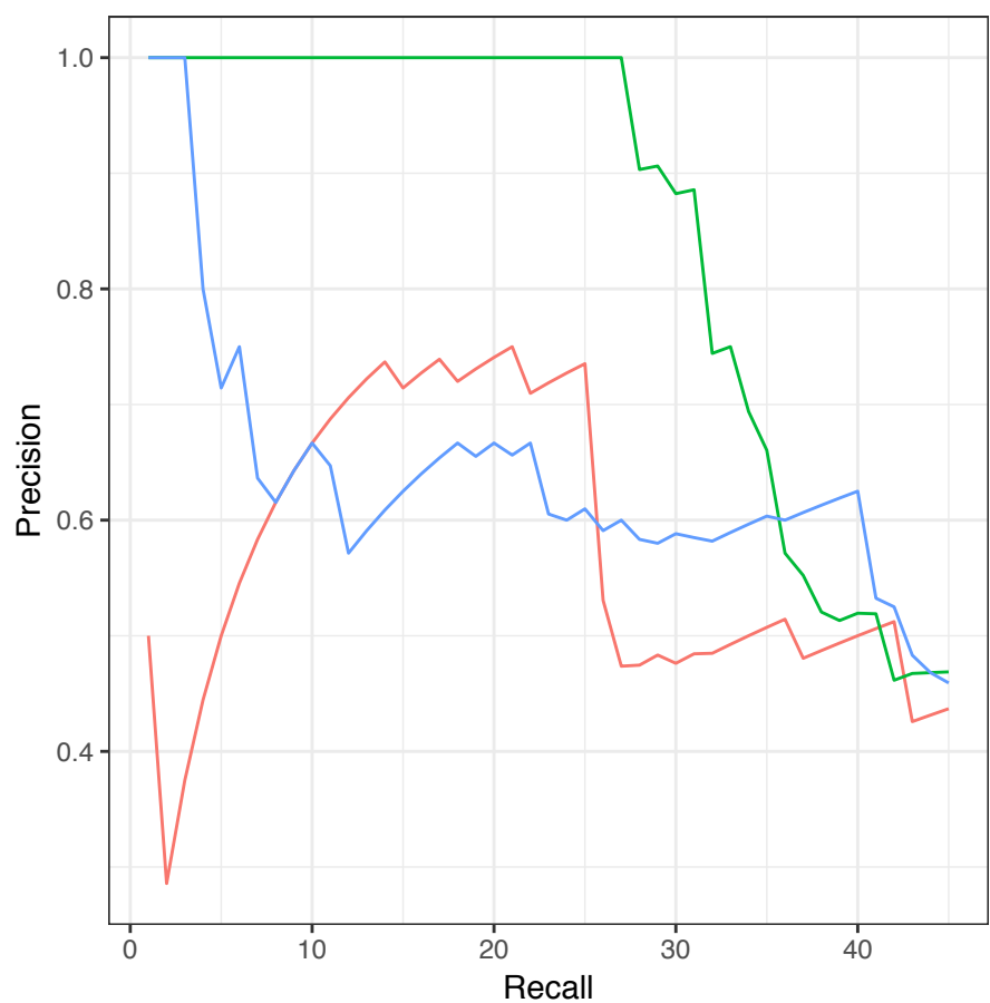
Precision-Recall curve for mouse Xist DMS AC
