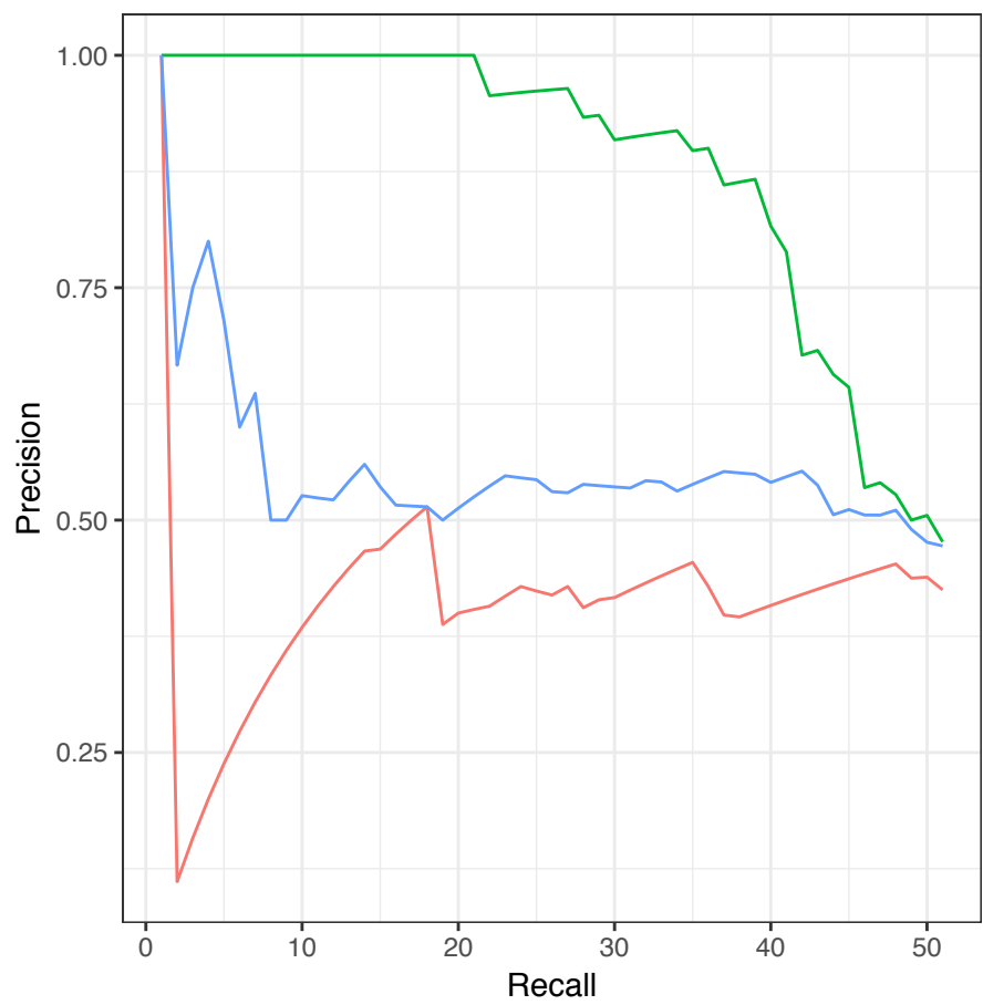
Precision-Recall curve for mouse 7SK DMS (primer 1) AC
