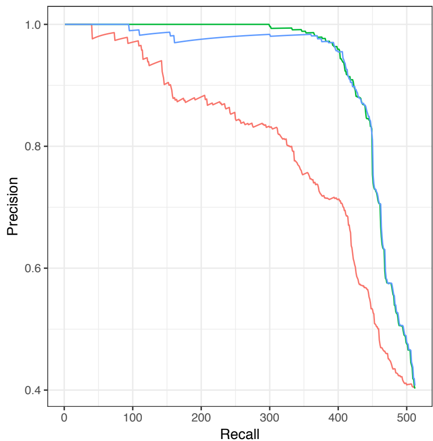
Precision-Recall curve for 5S rRNA SHAPE 2struct
