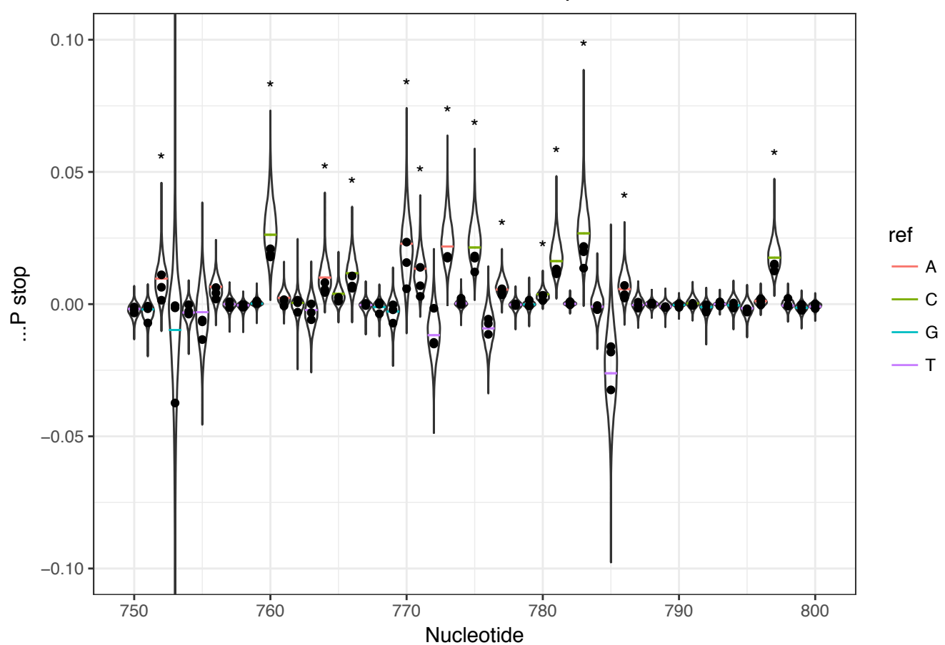
Inferred ...P distributions for 5S rRNA stops
