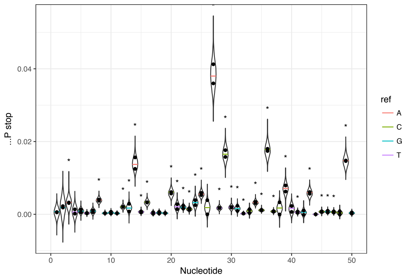
Inferred ...P distributions for mouse Xist stops
