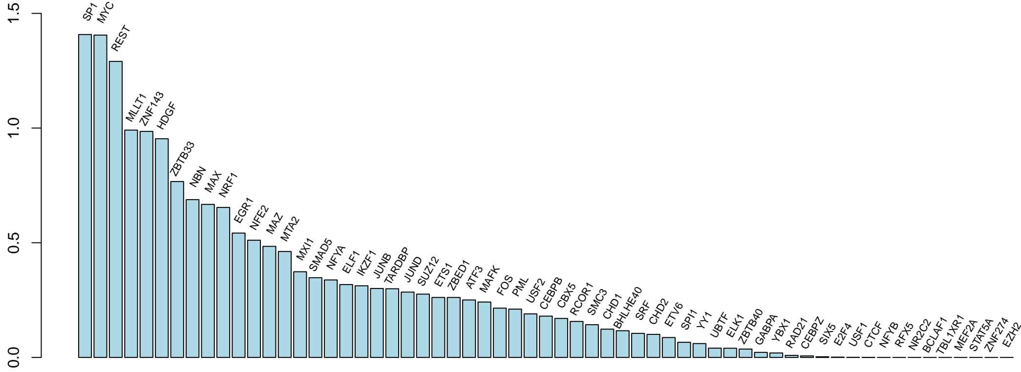
Hellinger Distance (GM versus K)
