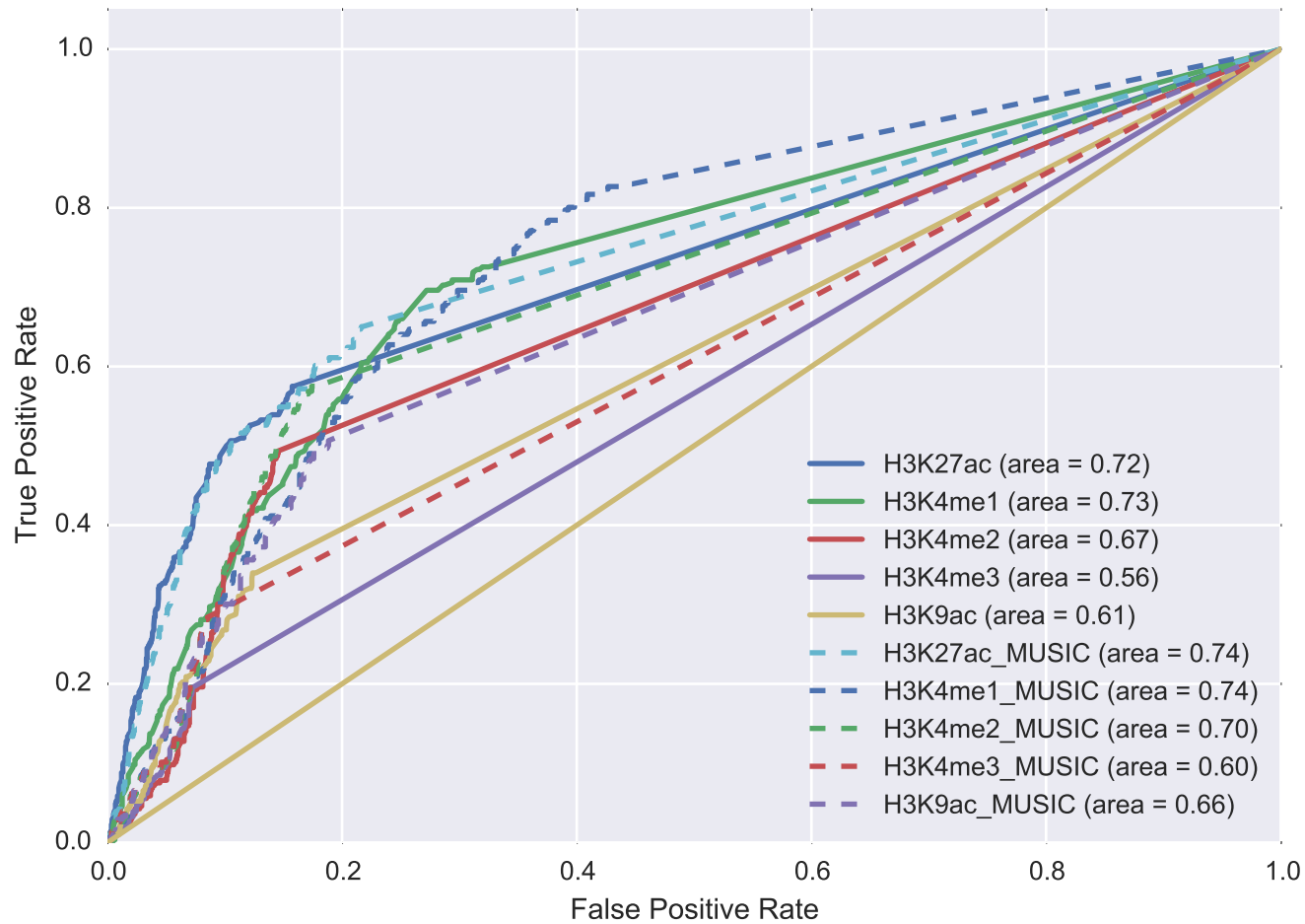
ROC Plot
