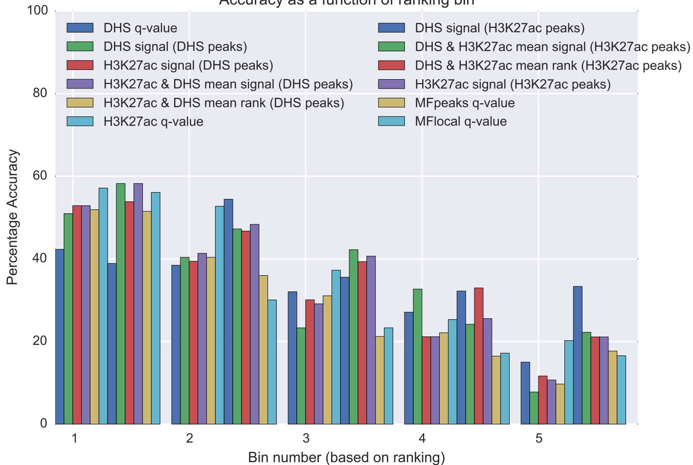
Accuracy as a function of ranking bin
