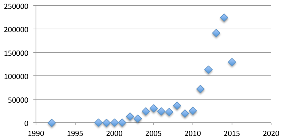
Eucaryotes - SIZE
