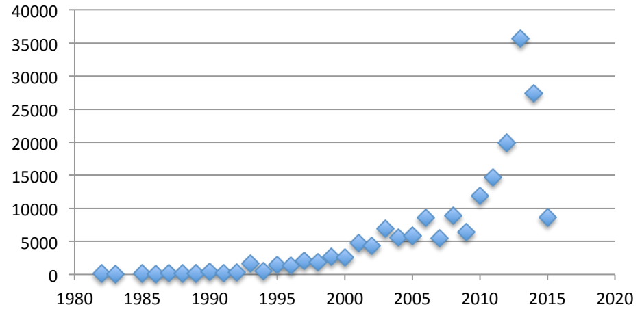
Viruses - SIZE
