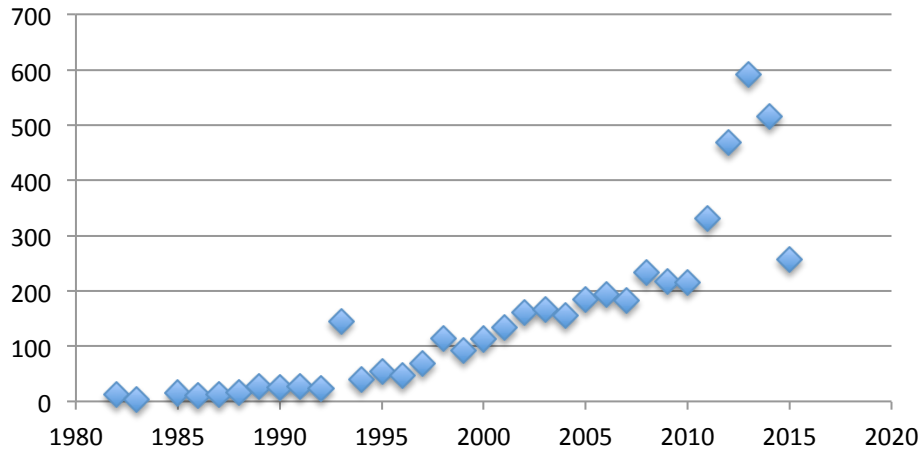
Viruses - #species
