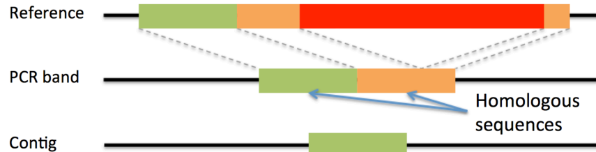
Figure S2. Examples of discrepancies in predicted and validated breakpoint coordinates. A) Most frequently, predicted breakpoints were shifted relative to those derived from validation excesses. One such example is depicted. All such cases were removed by post validation filteres. B) In one case (chr9:35803108-35803461) assembly collapsed tandem repeat around breakpoints resulting in shorter contig and overestimated breakpoints.
