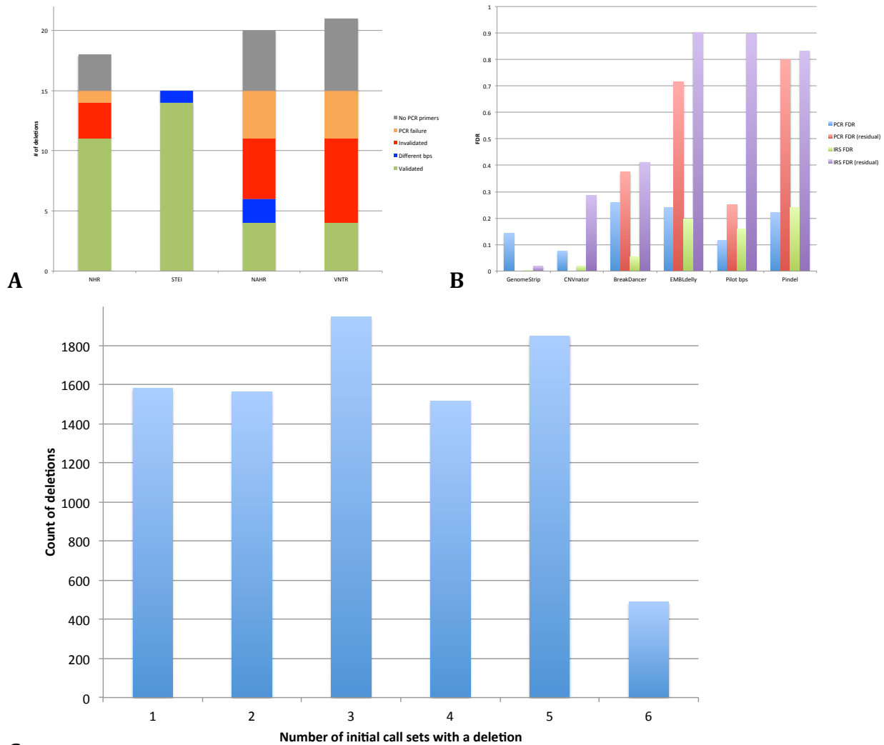
C Figure S5. Validation results before final deletion filtering. A) Breakdown by classification mechanisms. Deletions classified as Variable Number of Tandem Repeats – VNTR do not validate well as their breakpoints are in very repetitive sequences; B) Breakdown by calling method. Methods discovering deletions from split-read analysis (Delly, Pindel, and assembly in the pilot) have overall high FDR and very high residual FDR. C) Breakdown of deletions in the final set by presence in the initial call sets.
