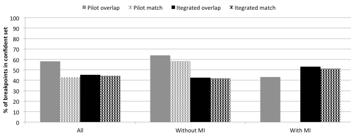
Figure S1. Comparison of confident set of breakpoints with pilot and integrated sets of breakpoints. A) Fraction of SV breakpoints that overlap 50% reciprocally between sets. B) Breakdown of confident breakpoints with/without MIs by 50% reciprocal overlap and exact match to breakpoints in pilot/integrated sets. For exact match we only matched start and end of the breakpoints. Overlap is higher with pilot set, but there is marked difference in the fraction of overlapping and exactly matching breakpoints to pilot set. The difference is particularly drastic for breakpoints with MIs, demonstrating that pilot set was particularly limited in resolving MIs. The difference is minor when comparing to integrated set. However, integrated set represented deletion breakpoint in a narrow size range (Fig. 1C).
