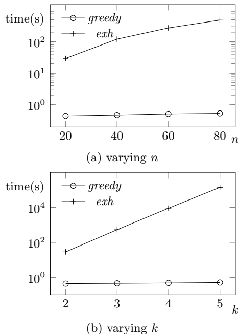
Figure 2: Running time: greedy vs. exh
