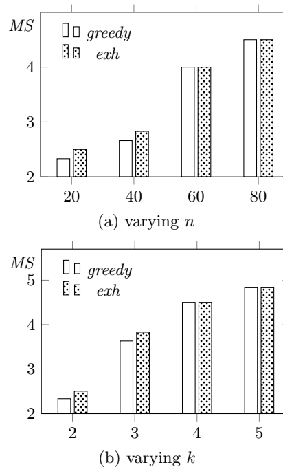
Figure 3: Market share (%): greedy vs. exh
