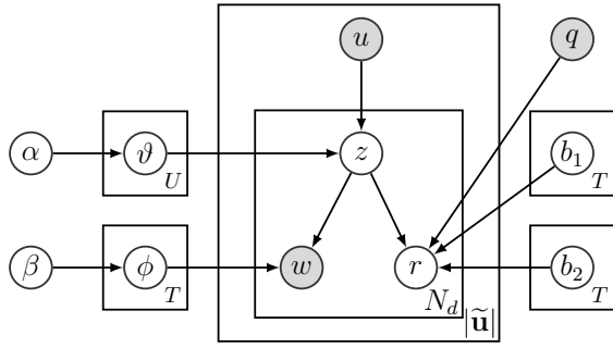
Figure 1: Graphical representation of user-interest topic model.
