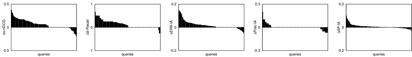
Figure 2: Per query performance differences of PSVM_{div} against SVM_{div} . The figures shown are for \alpha -nDCG, S-Recall, ERR-IA, Prec-IA and MAP-IA, respectively. A bar extending above the center of a plot indicates that PSVM_{div} outperforms SVM_{div} , and vice versa for bars extending below the center. Note that figures are not in the same scale.
