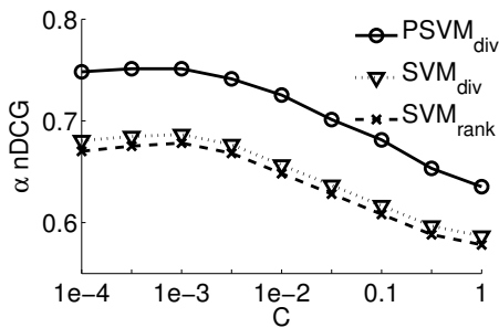
Figure 4: Performance of the supervised methods using all features when varying the value of parameter C .
