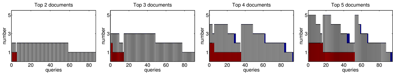
Figure 3: How runs produced by PSVM_{div} and SVM_{div} differ. Red, white, blue bars indicate the number of different subtopics that appear in PSVM_{div} but not in SVM_{div} , in both runs and not in PSVM_{div} but in SVM_{div} , respectively, at corresponding depth k (for k=2, 3, 4, 5 ). Figures should be viewed in color.
