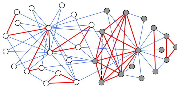
Figure 2: Karate Club graph. Blue light edges represent the weak edges, red thick edges represent the strong edges, and the black dashed edge represents the added edge
