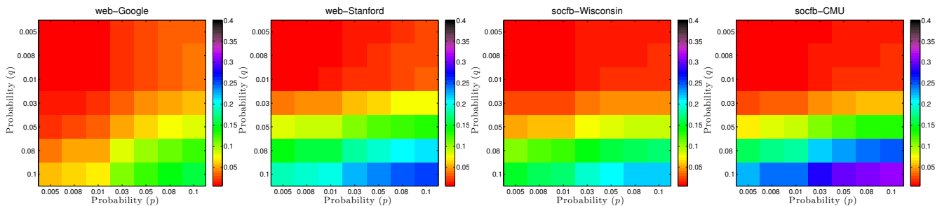
Figure 2: Sampling Fraction ( \frac{\text{SSize}}{N_K} ) as p, q changes in the range ‘0.005–0.1’ for web and social graphs (ordered from sparse → dense).
