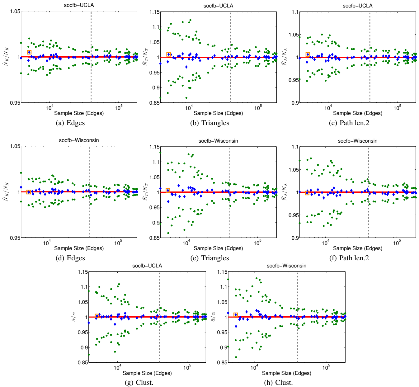
Figure 1: Convergence of the estimates ( N_K , N_T , N_A , \alpha , upper and lower bounds) for socfb-UCLA and socfb-Wisconsin graphs, for all possible samples with p, q in the range 0.005–0.1. Diamonds (Blue): \frac{E[\text{est}]}{\text{Actual}} . Circles (Green): \frac{\text{UB}}{\text{Actual}} , \frac{\text{LB}}{\text{Actual}} . Square (Orange): refers to the sample in Table 3. Dashed vertical line (Grey): refers to the sample at 40K edges
