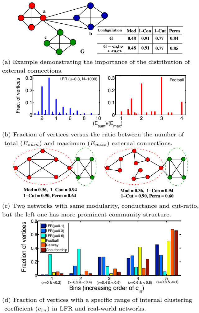
Figure 1: (Color online) Toy examples and empirical observations demonstrating the drawbacks of existing community scoring metrics. The communities in (a) and (c) are distinguished by different colors.
