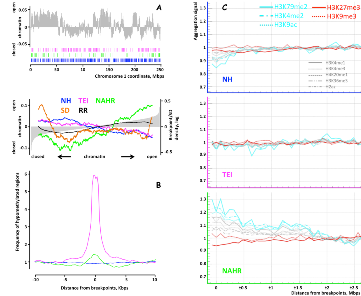
Figure 3. Relation of breakpoints of each class to chromatin states, histone marks and methylation. A) Breakpoint co-occurrence with chromatin states, defined by corresponding eigenvector, of Hi-C data (upper panel). The genome wide co-occurrence is ordered by the value of the eigenvector (lower panel). Curves were smoothed using sliding window of 3,000 bins. NAHR breakpoints are associated with open chromatin. This association cannot be explained by higher content of segments duplications (SDs) or recombination rate (RR). B) Overlap of breakpoints with hypomethylated regions in sperm. NAHR and TEI breakpoints show strong association. C) Association with histone marks. NH breakpoints were depleted for all active marks and also for the H3K9me3 repressive mark (red lines). TEI breakpoints showed weak depletion of active marks. While the density of repressive H3K27me3 mark decreases close to NAHR breakpoints, the density of all active marks increase.
