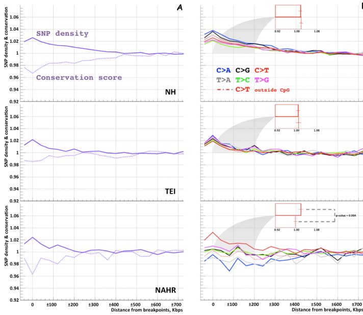
Figure 2. Co-aggregation of SNPs with deletion breakpoints found in the analyzed samples. A) Normalized by nucleotide frequency and background SNP densities increased while conservation decreased in 400 kbp regions around breakpoints of each class. B) Densities increase for substitutions of all types around NH and TEI breakpoints but this is not the case for NAHR breakpoints. Increase of C to T substitutions around NAHR breakpoints is driven by SNPs in CpG motifs as evident from red bars. Furthermore, this is solely due to enrichment of CpG motifs (Fig. S2). This is consistent with common knowledge that NAHR events are associated with sites of recombination.
