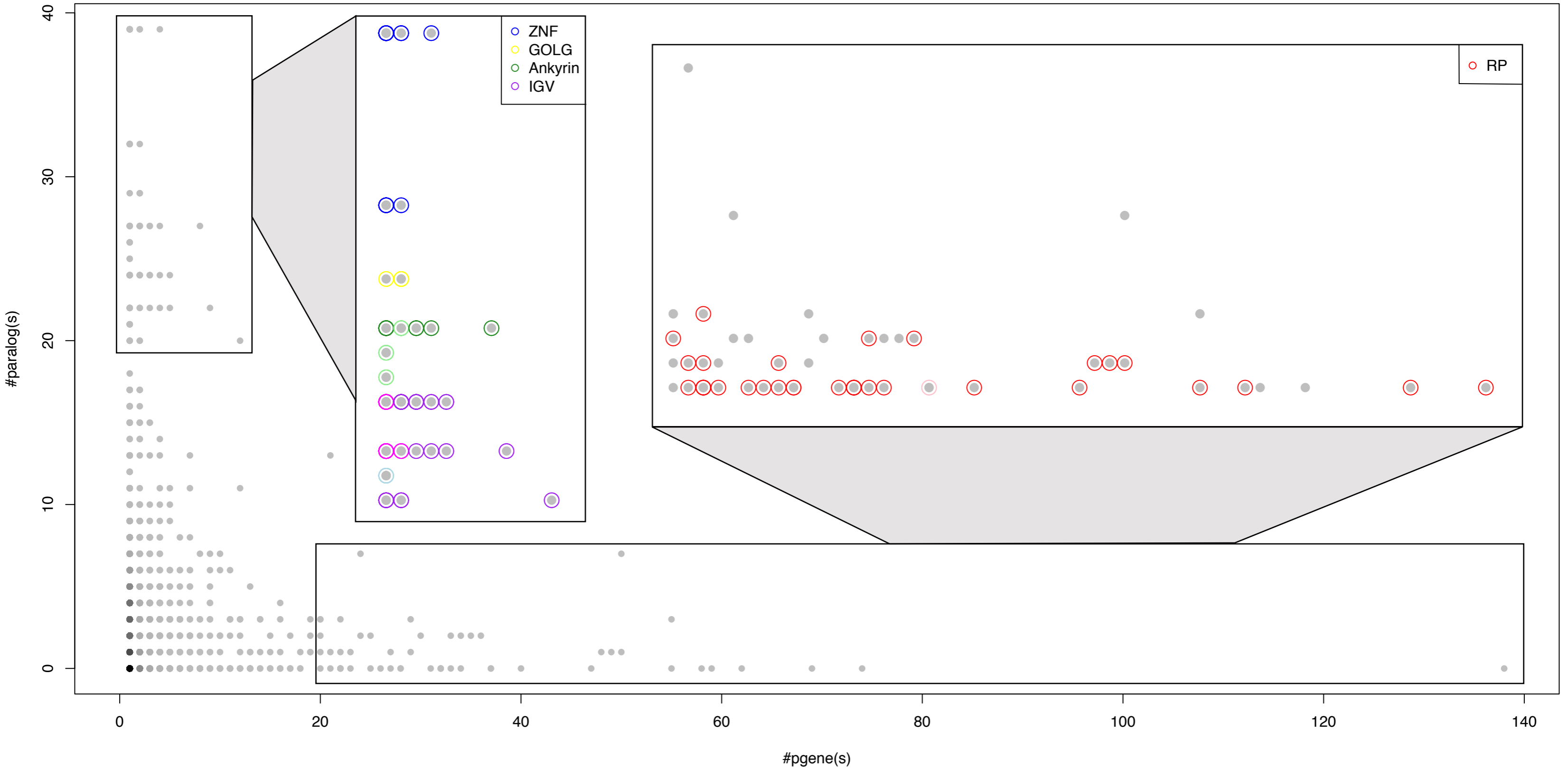
Human 3857 transcripts w/pgene(s)
