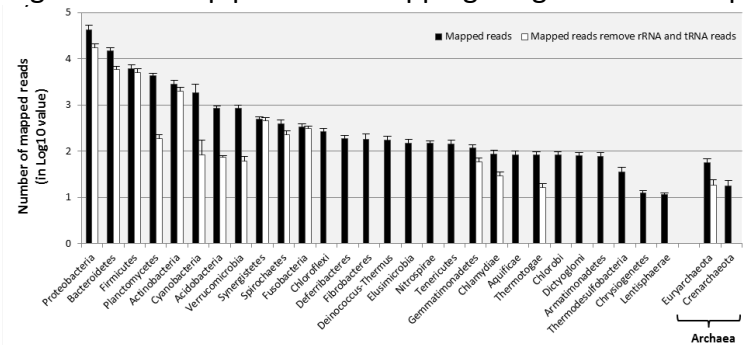
Figure 2. Mapped reads to microbial genera, using initial pipeline.
