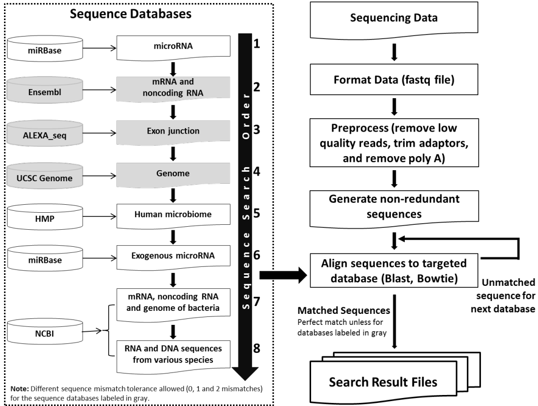
Figure 1. Initial pipeline for mapping exogenous RNA in plasma.
