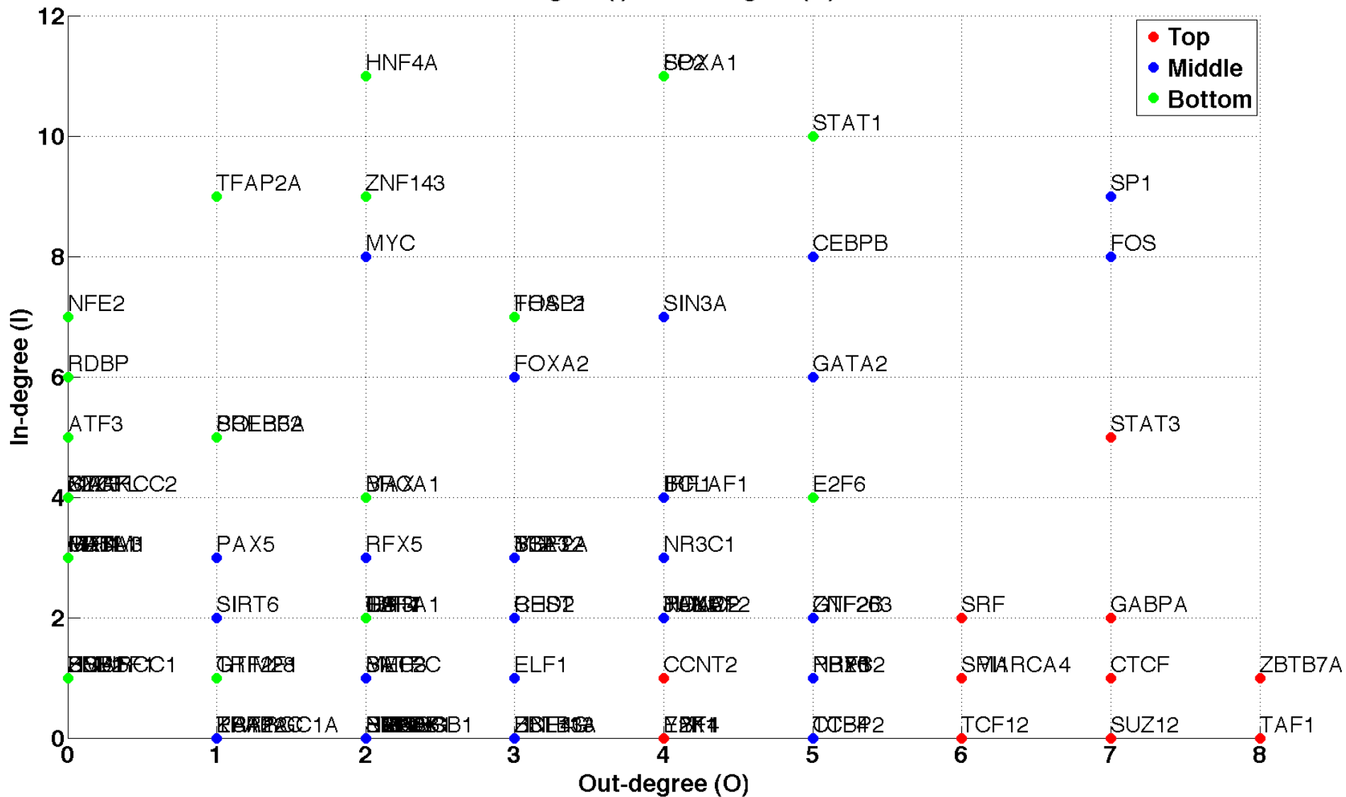
In-degree (I) vs out-degree (O)
