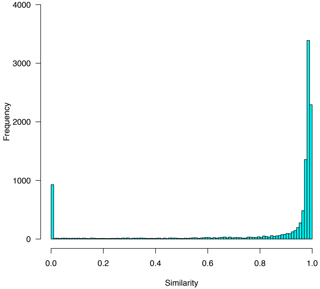
Histogram of sequence similarity to Chimp -- all pgenes
