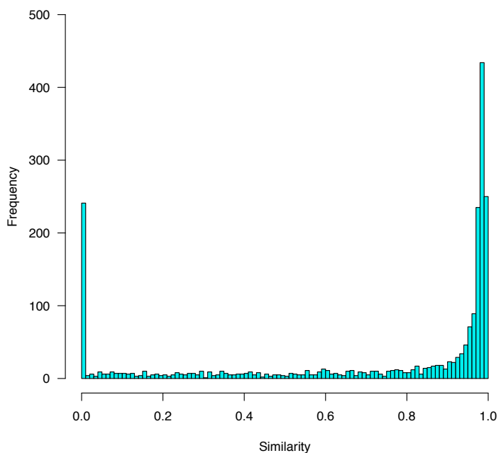
Histogram of sequence similarity to Chimp -- transcribed pgenes
