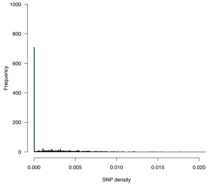
Histogram of SNP density -- Transcribed pgenes
