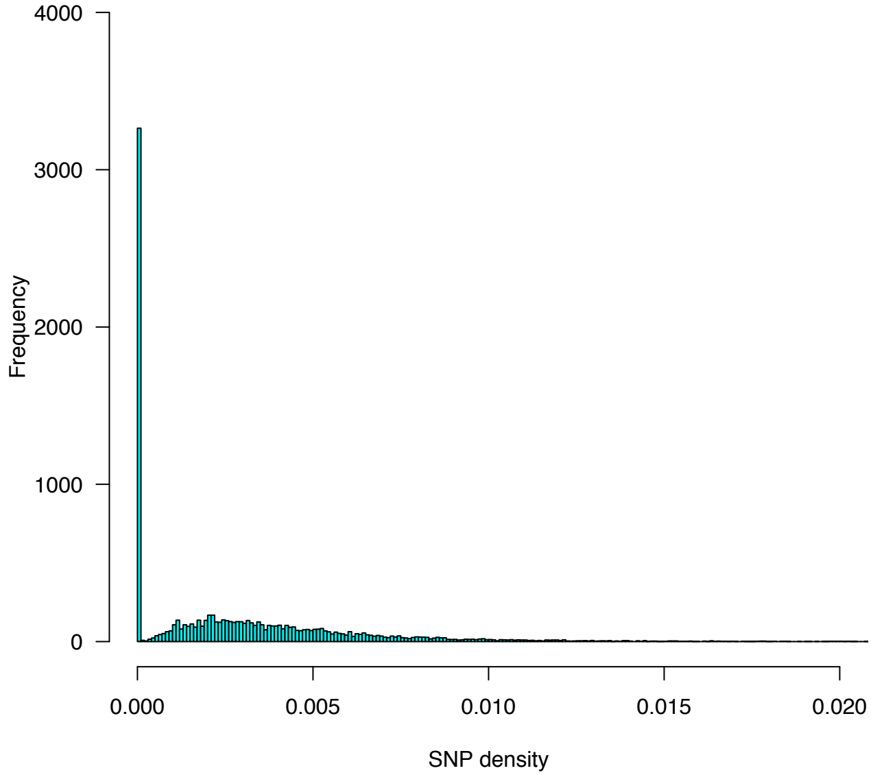
Histogram of SNP density -- All pgenes
