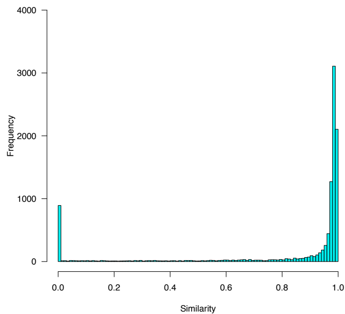
Histogram of sequence similarity to Chimp -- non-Transcribed pgenes
